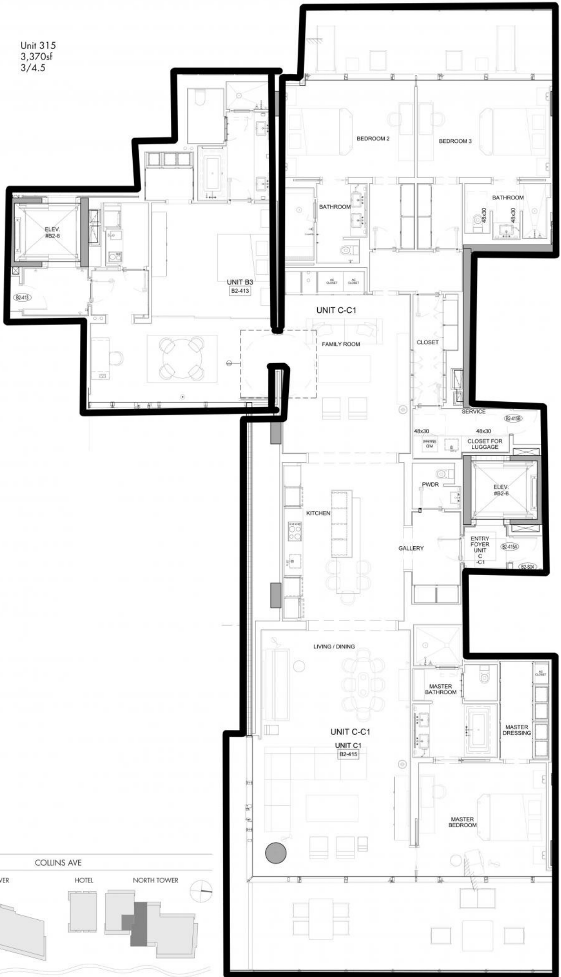
1 ENLARGED UNIT PLAN - UNIT B3 & C1
